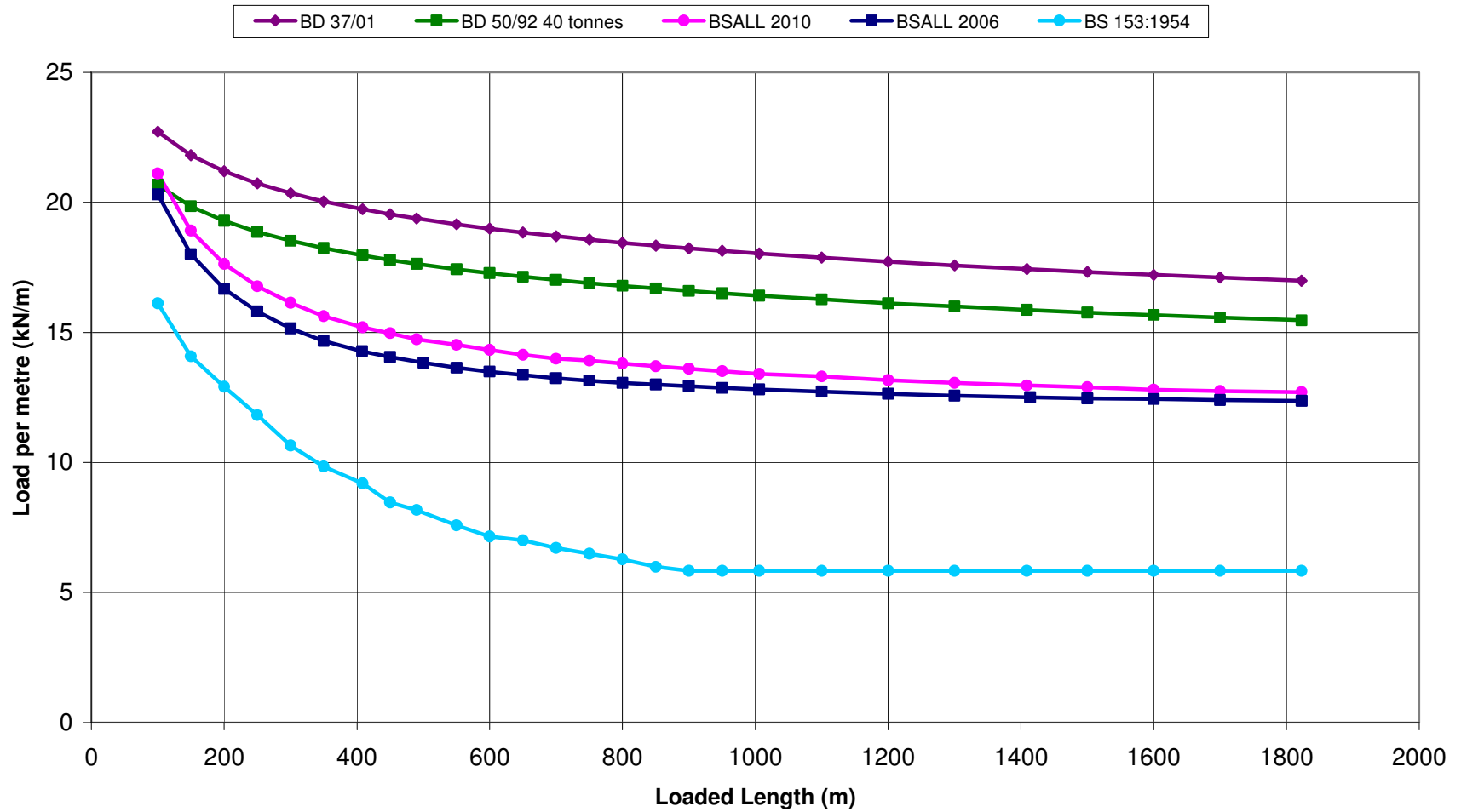
Figure 2 : Recommended Assessment Loading (Nominal) - Lane 1
